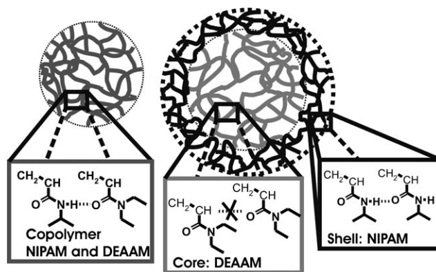
Figure 1. The different microgel types, copolymer (left) versus core-shell (right), and the intramolecular hydrogen bonds. The third system (PNIPAM core and poly( N,N -diethylacrylamide) (PDEAAM) shell) is not shown.
